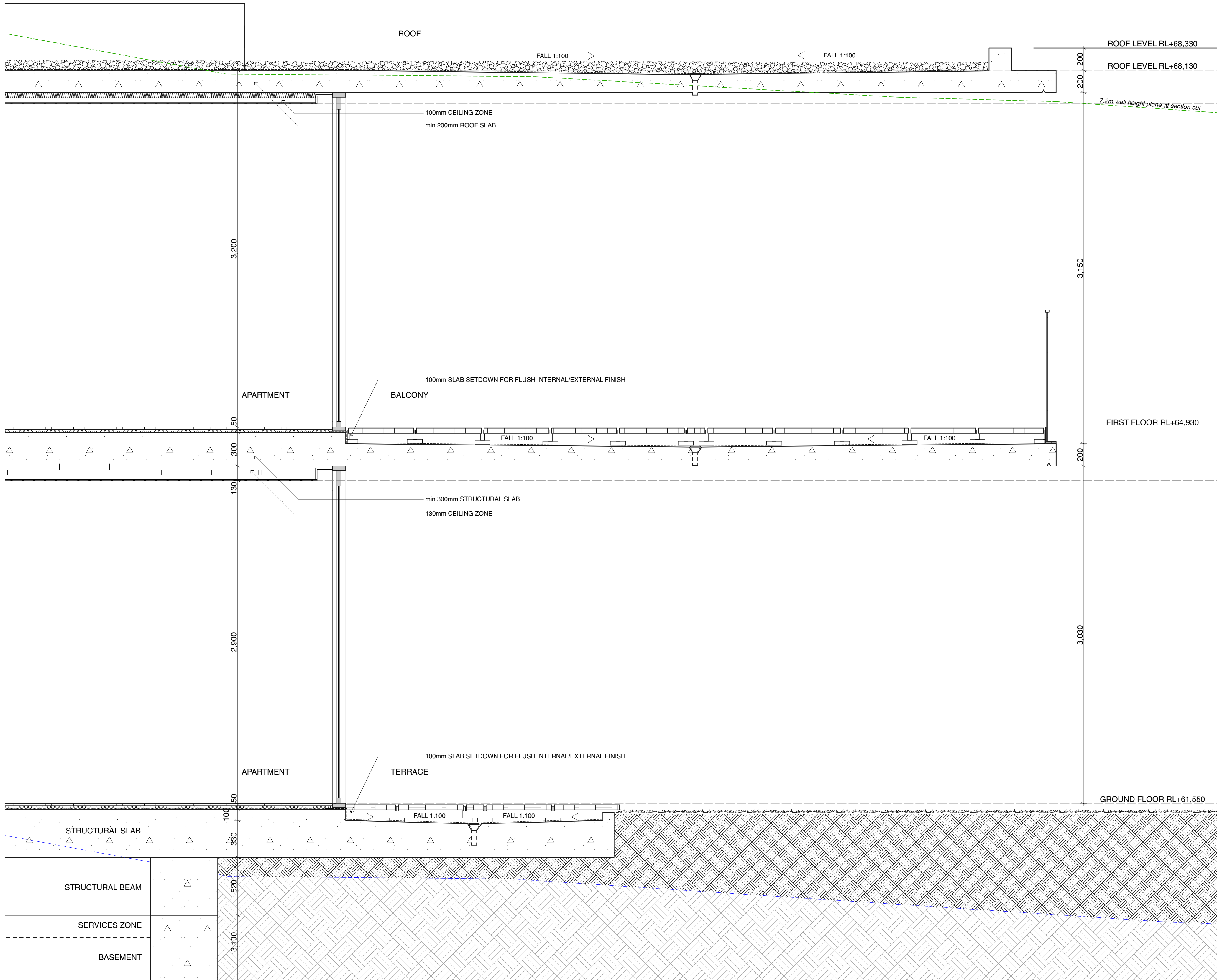
SECTION DETAIL 1
