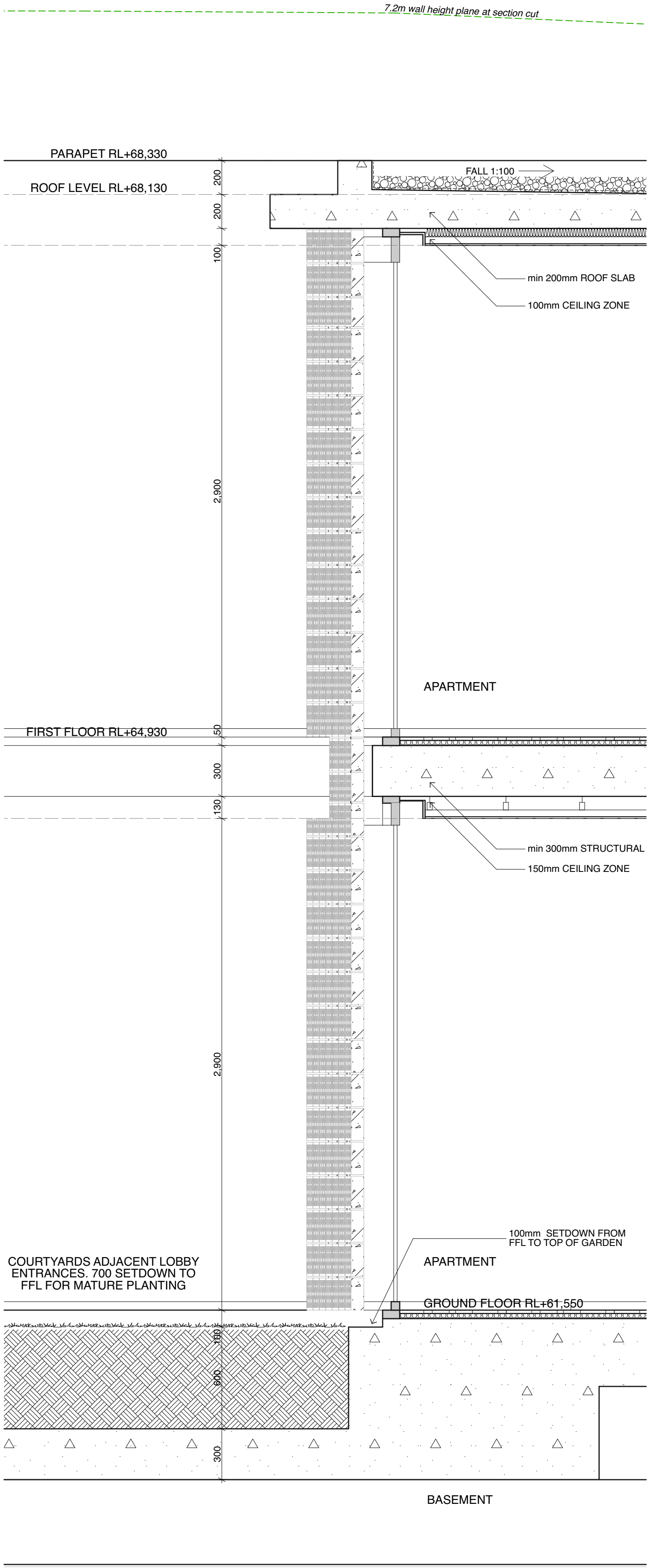
SECTION DETAIL 2
